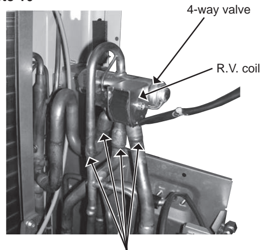
Brazed parts
