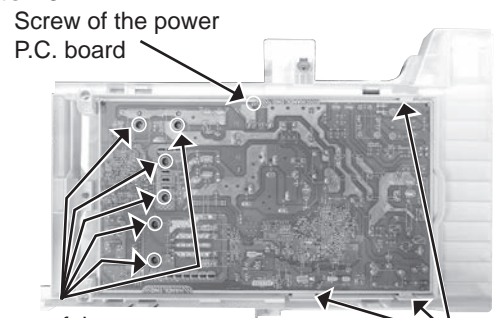
Screws of the power P.C. board and the heatsink
